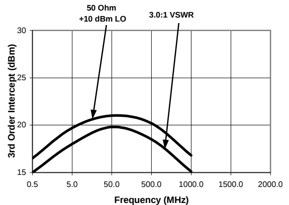
3rd Order intercept vs. IF Port Termination
